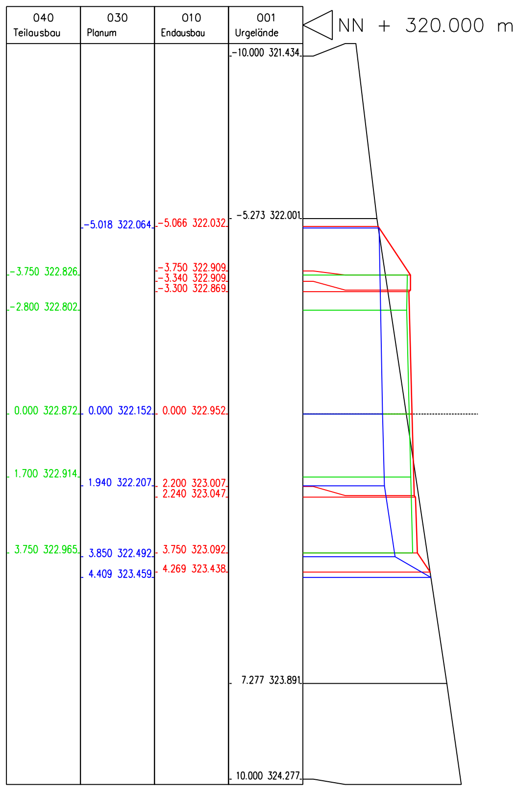
Station 120,000
