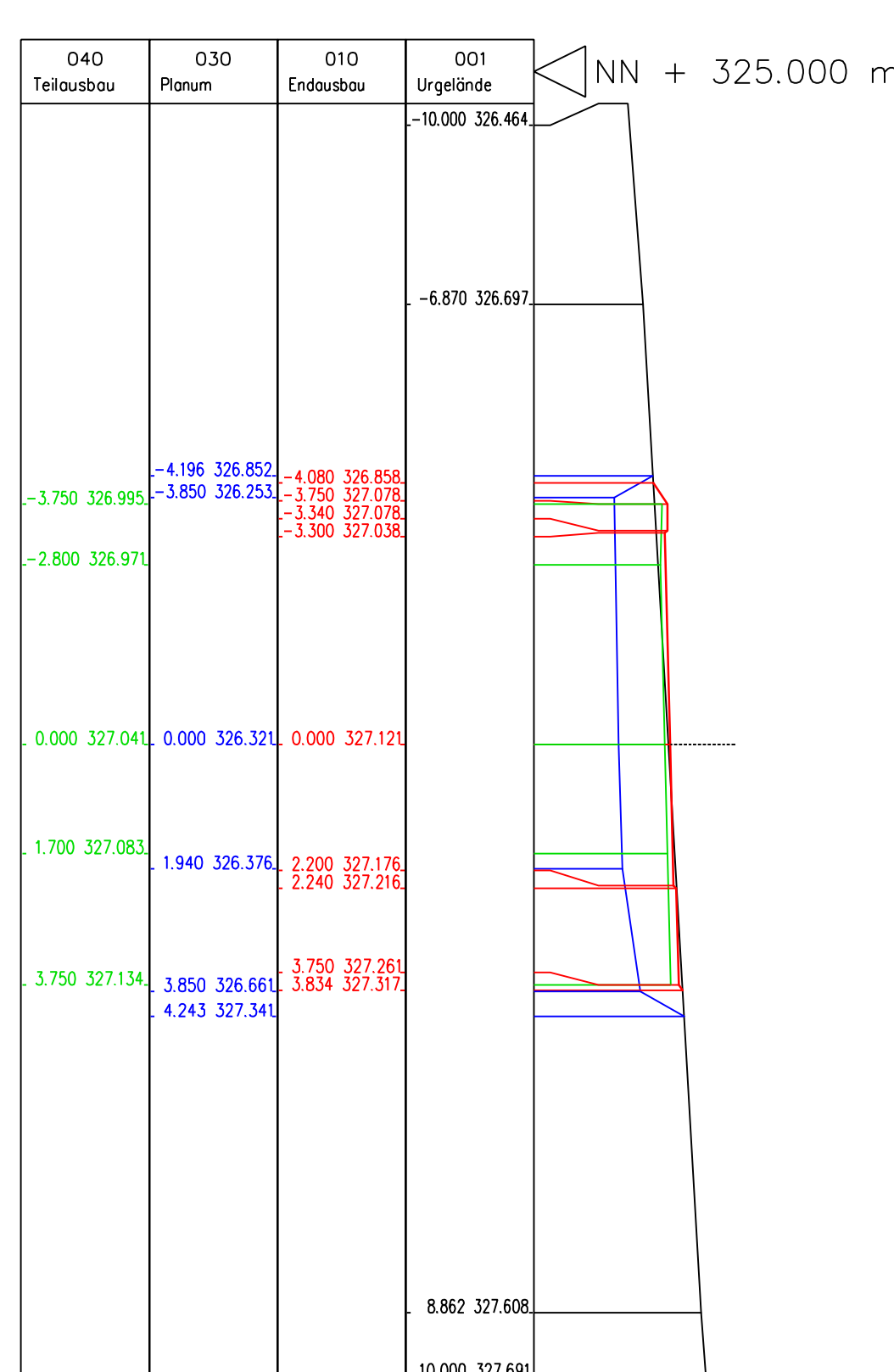
Station 40,000
