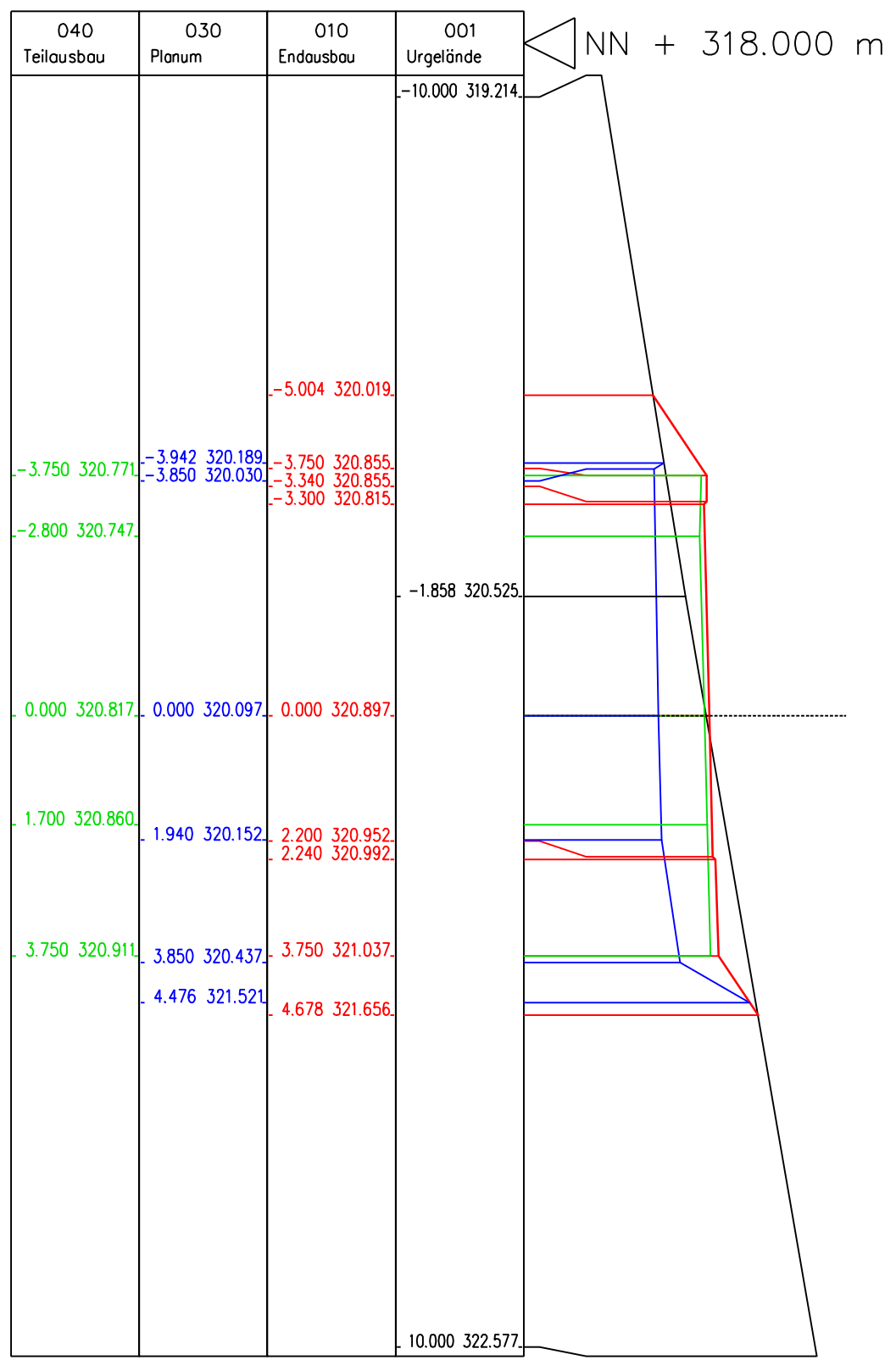
Station 170,342
