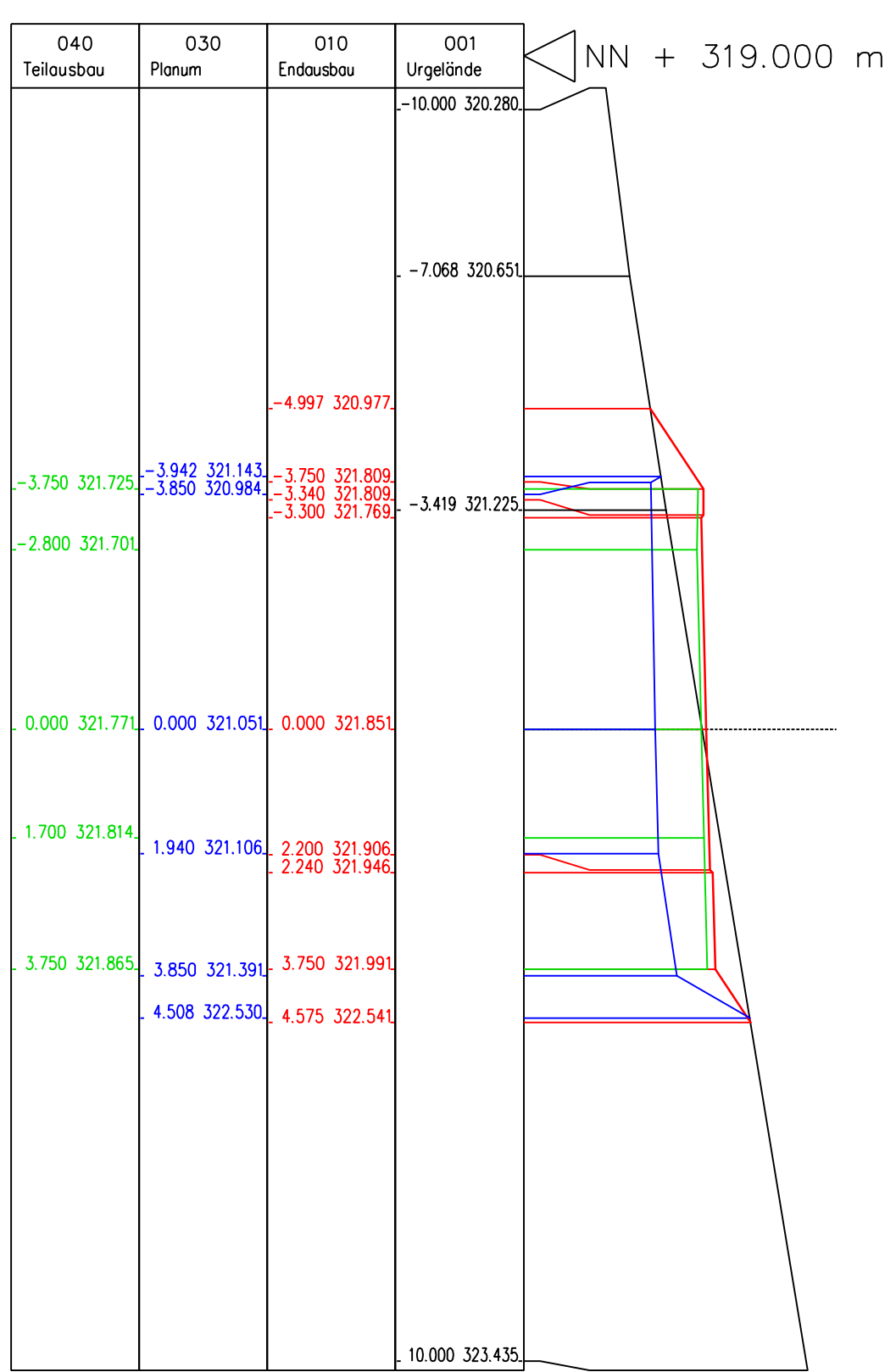
Station 140,000
