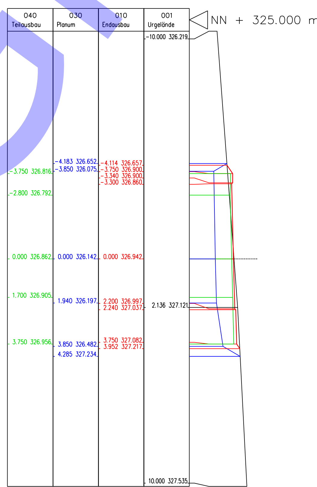
Station 20,000
