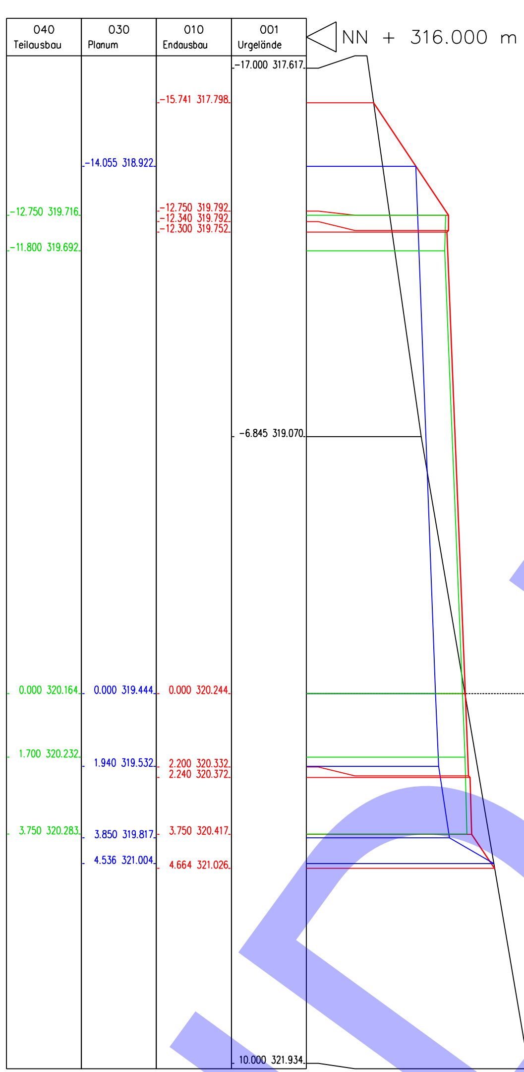
Station 191,642
